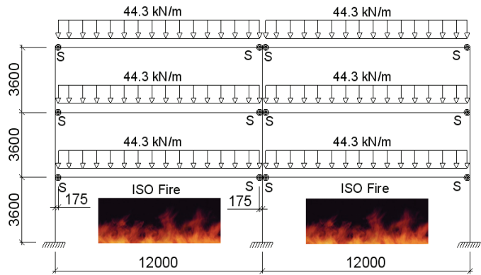
Figure 1. Considered frame.
