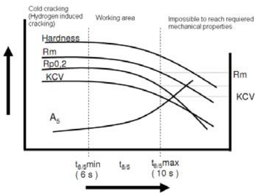
Fig. 5 – Influence of cooling rate on mechanical properties of weld [3]
